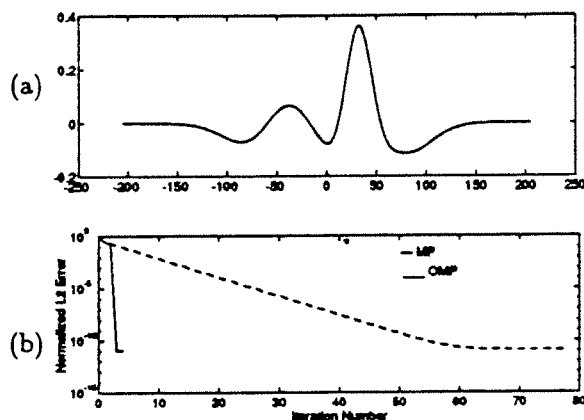
Figure 5: Example II: (a) Original signal f , (b) Squared L^2 norm of residual R_k f versus iteration number k , for both OMP (solid line) and MP (dashed line).
